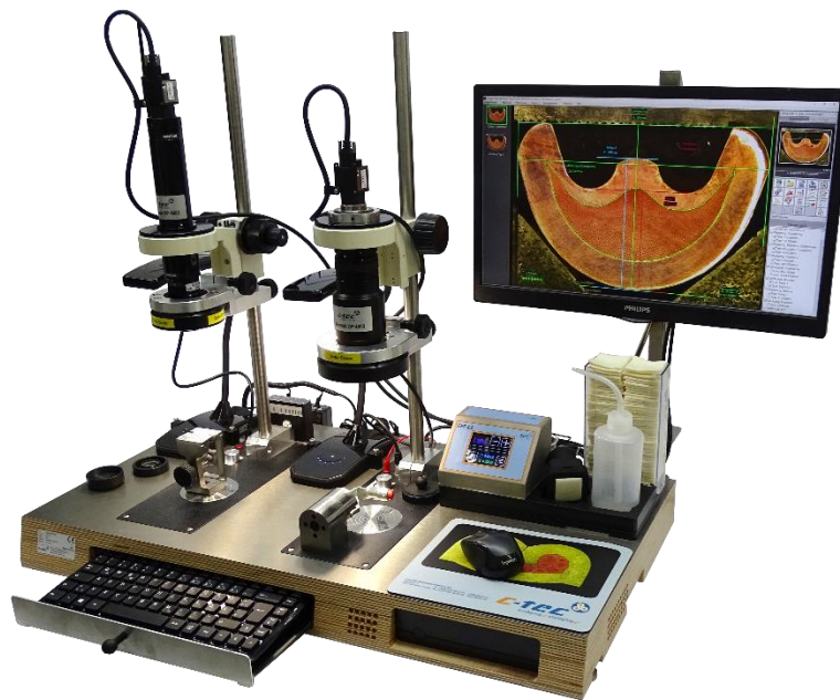
Dual optic station OP 4003-pc with optional EFP 4.0
