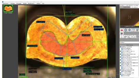
Finished microsection with X-Scan
